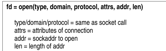
Figure 12: New open
