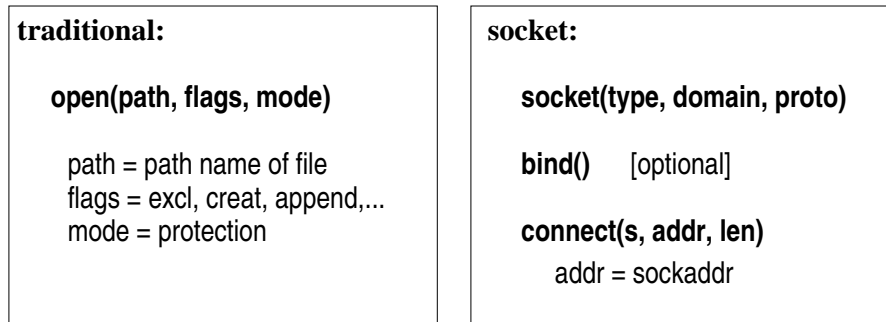
Figure 11: Opens
