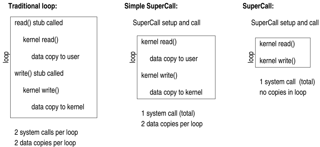
Figure 14: SuperCall
