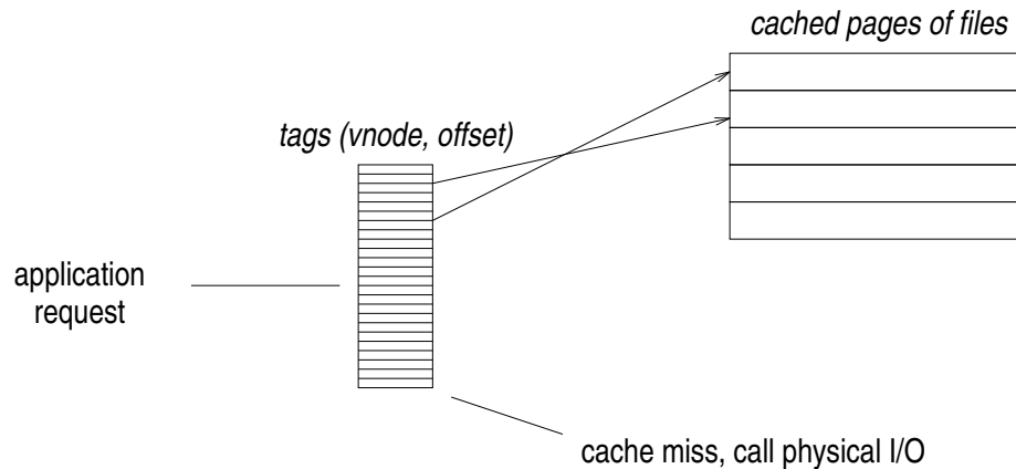
Figure 18: File cache
