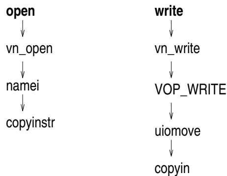
Figure 15: Copy depth
