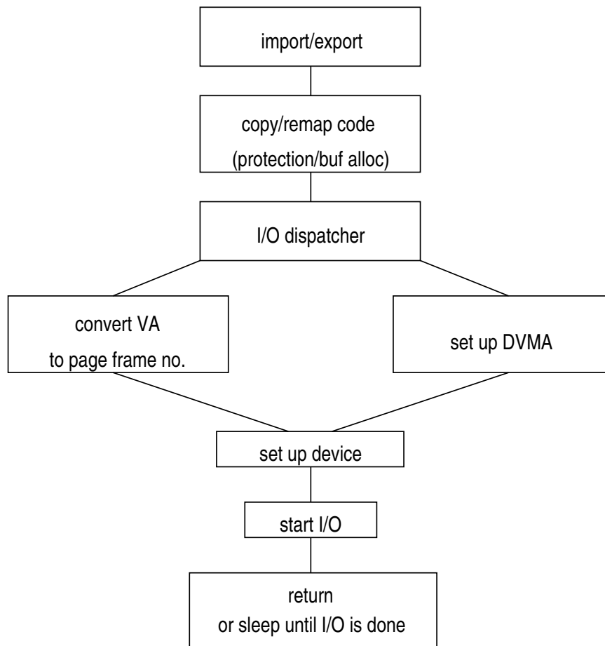
Figure 16: VM operations
