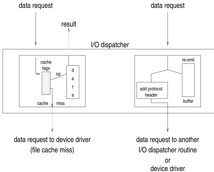
Figure 17: Two example paths through the I/O Dispatcher
