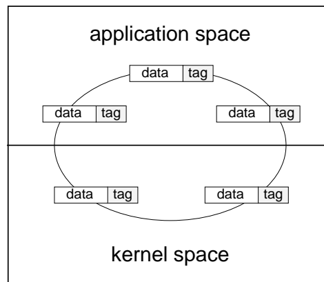
Figure 6: A pool of buffers
